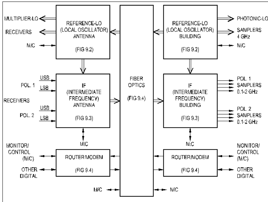
Figure 9.1: Reference-LO IF and FO Systems
