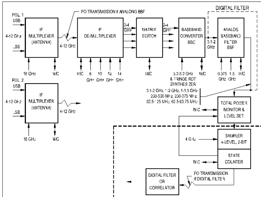
Figure 9.3: IF System (Intermediate Frequency)
