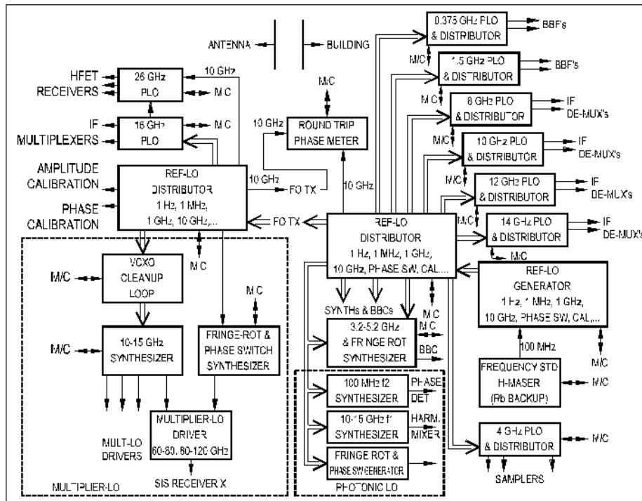
Figure 9.2: Reference-LO System (Local Oscillator)
