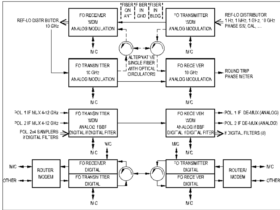
Figure 9.4: FO System (Fiber Optic)
